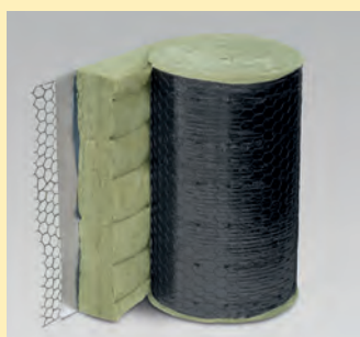
U Protect Wired Mat 4.0 Alu1 Wired Mat: L x 600 mm Facing: aluminium
